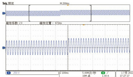
AC+DC: 220VAC叠加100VDC
