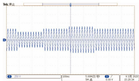
IEC61000-4-14电压波动
